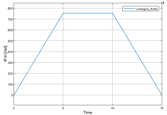
Figura 40: Consigna \theta_m^*
